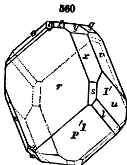
Cornwall.
